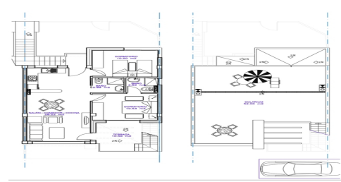
General property plan Top floor
